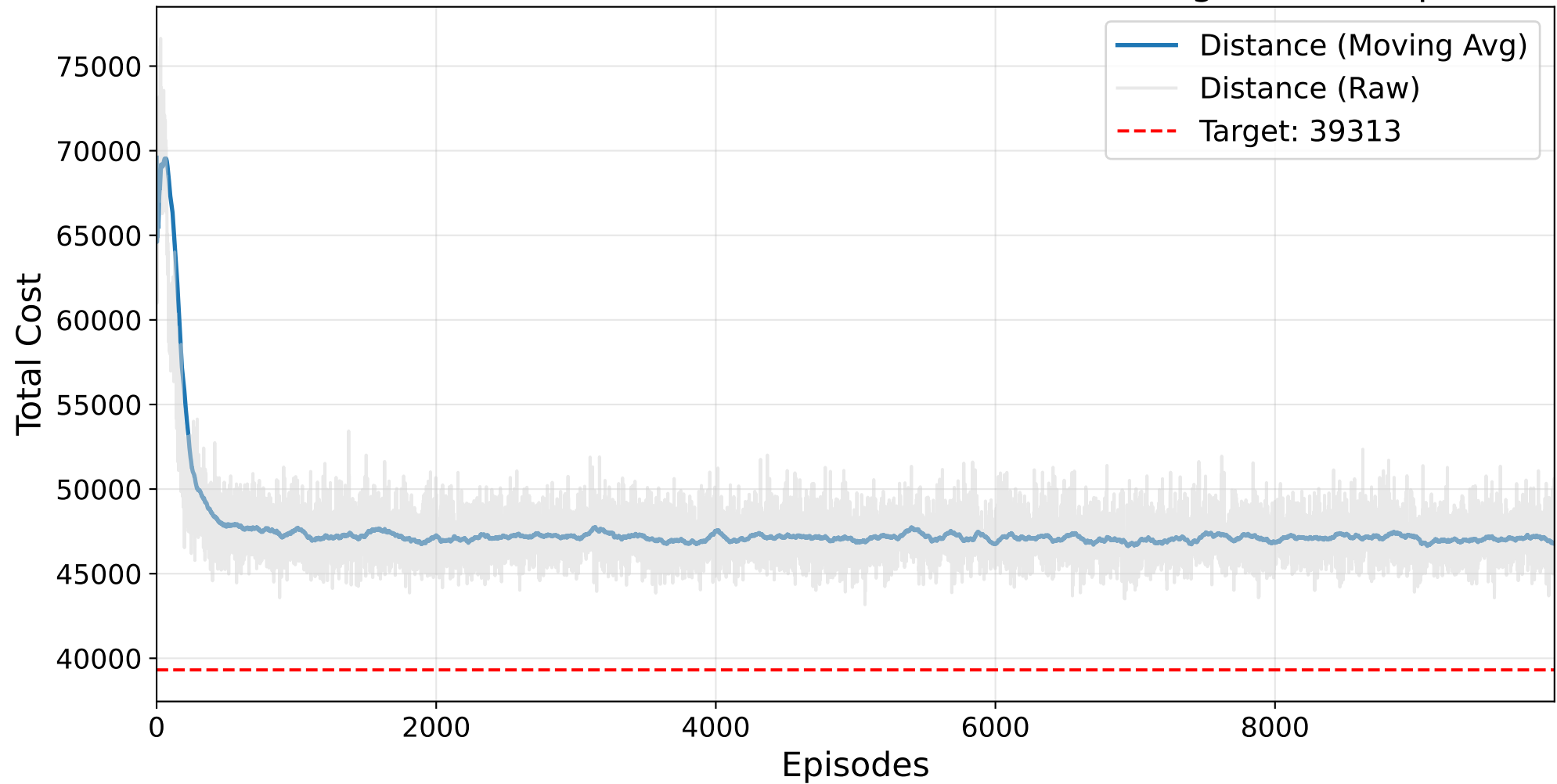
Final HYPERBAND GP Masked AutoRL-SOP Training - ft70.1.sop
